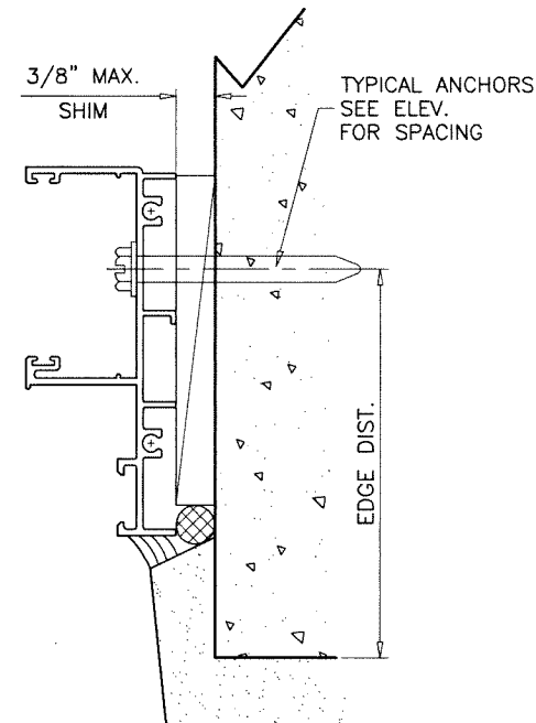
FLUSH FRAME WITH TRIMMED EXTERIOR FLANGE HEAD/SILL/JAMB
